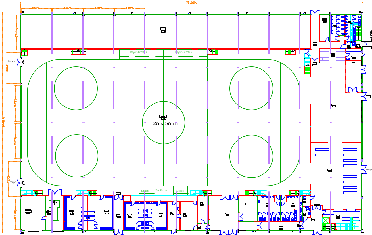
Plan ground floor
